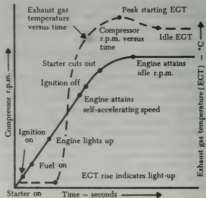
FIGURE 5-11. Typical gas turbine engine starting sequence.
